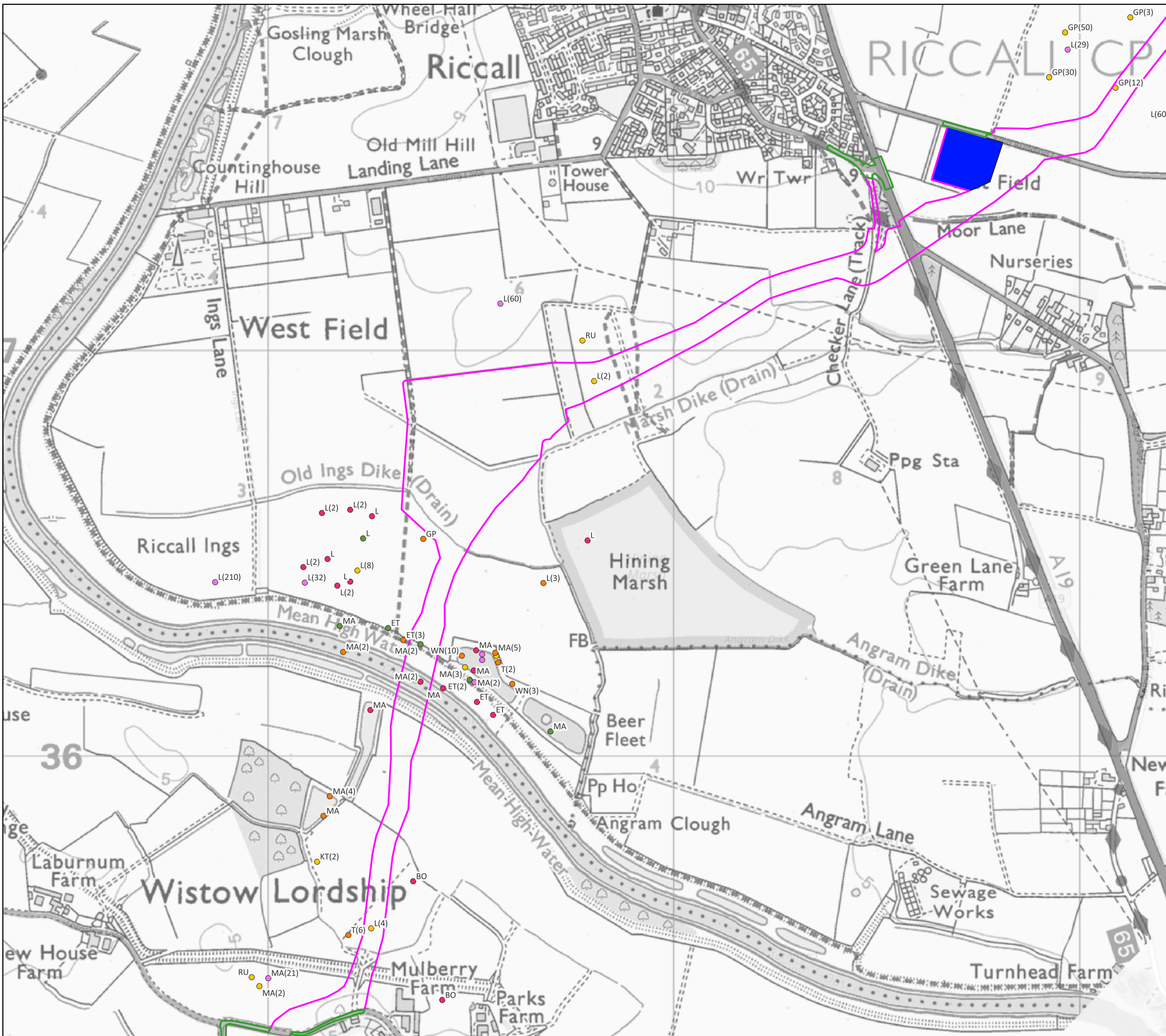
Figure 16: Non-Breeding Bird Results - Birds on the Ground Cable Route - Map 4
