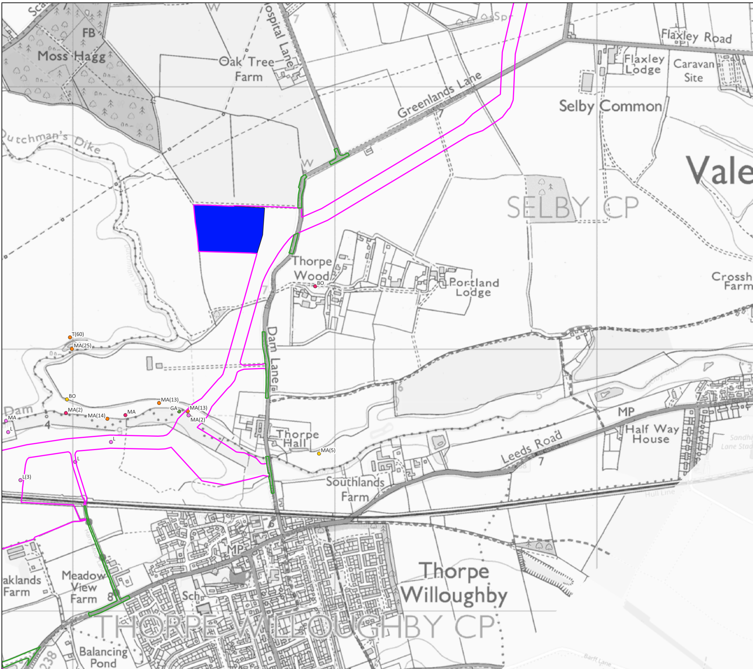
Figure 19: Non-Breeding Bird Results - Birds on the Ground Cable Route - Map 7
