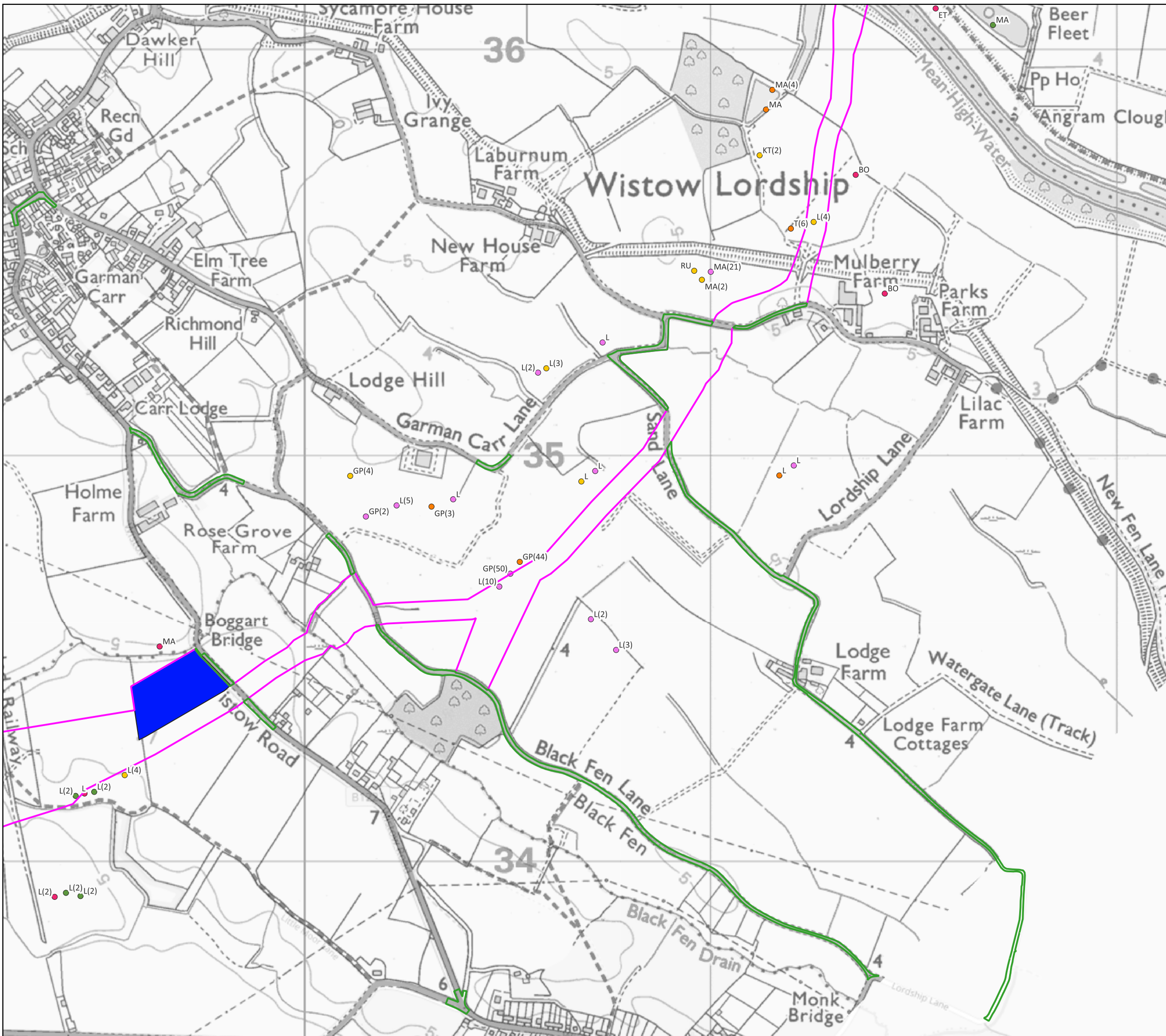
Figure 17: Non-Breeding Bird Results - Birds on the Ground Cable Route - Map 5
