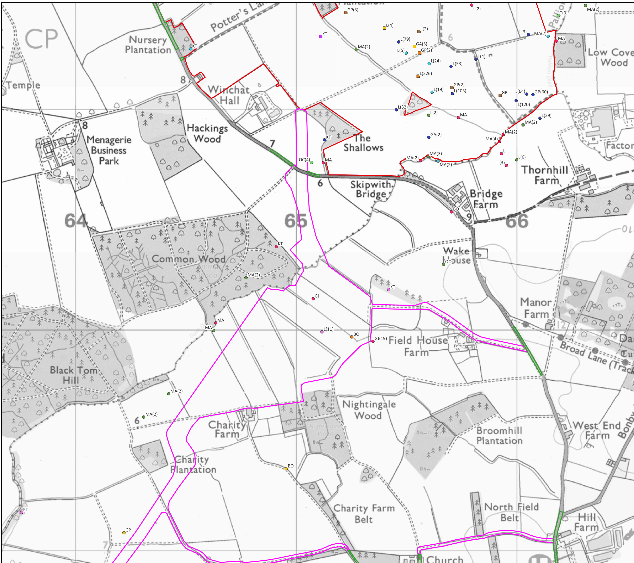
Figure 13: Non-Breeding Bird Results - Birds on the Ground Cable Route - Map 1
