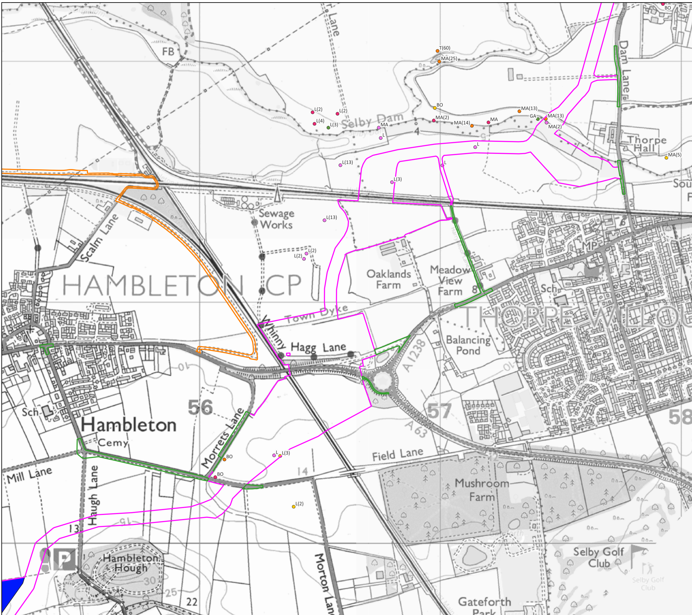
Figure 20: Non-Breeding Bird Results - Birds on the Ground Cable Route - Map 8
