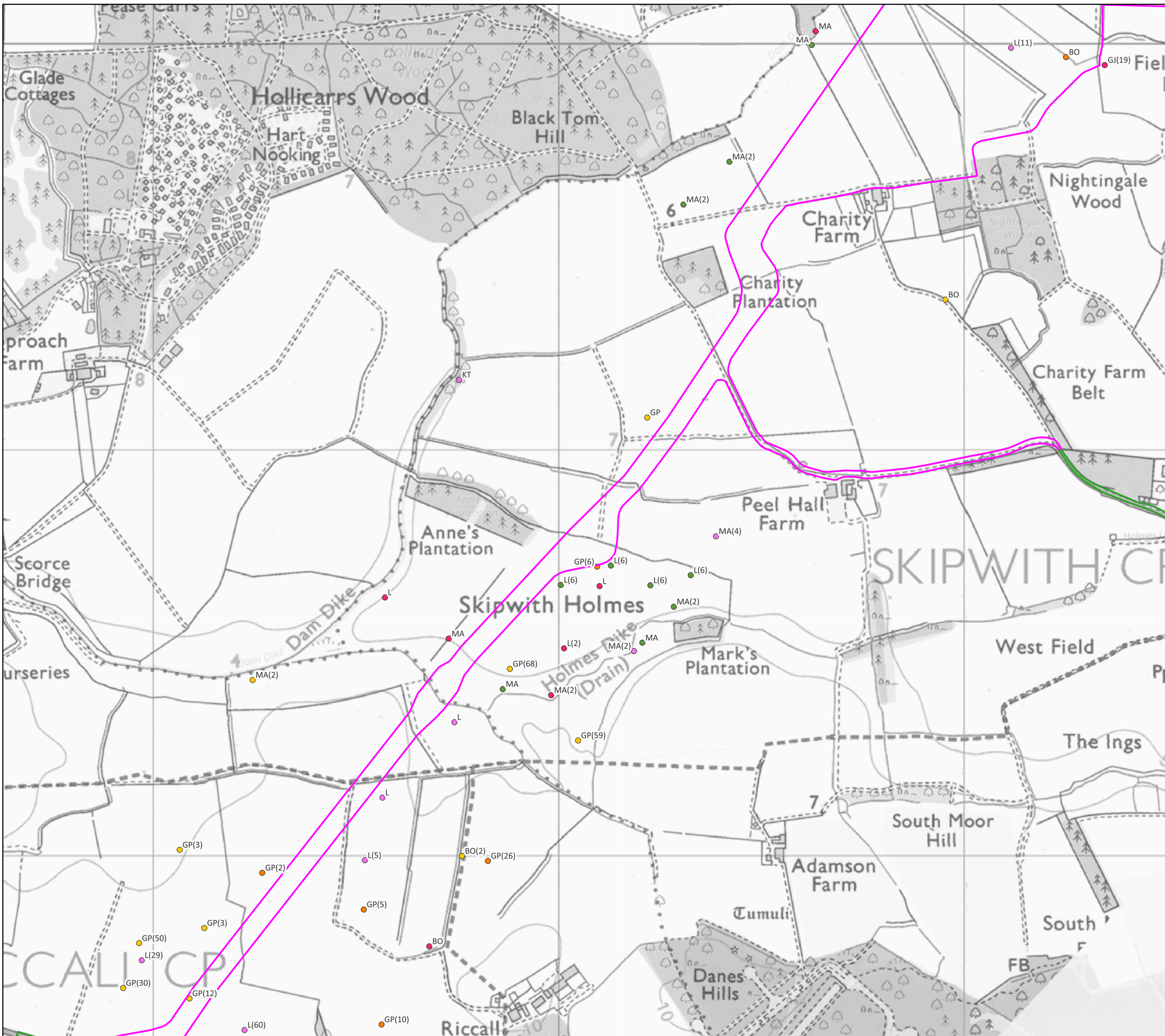
Figure 14: Non-Breeding Bird Results - Birds on the Ground Cable Route - Map 2
