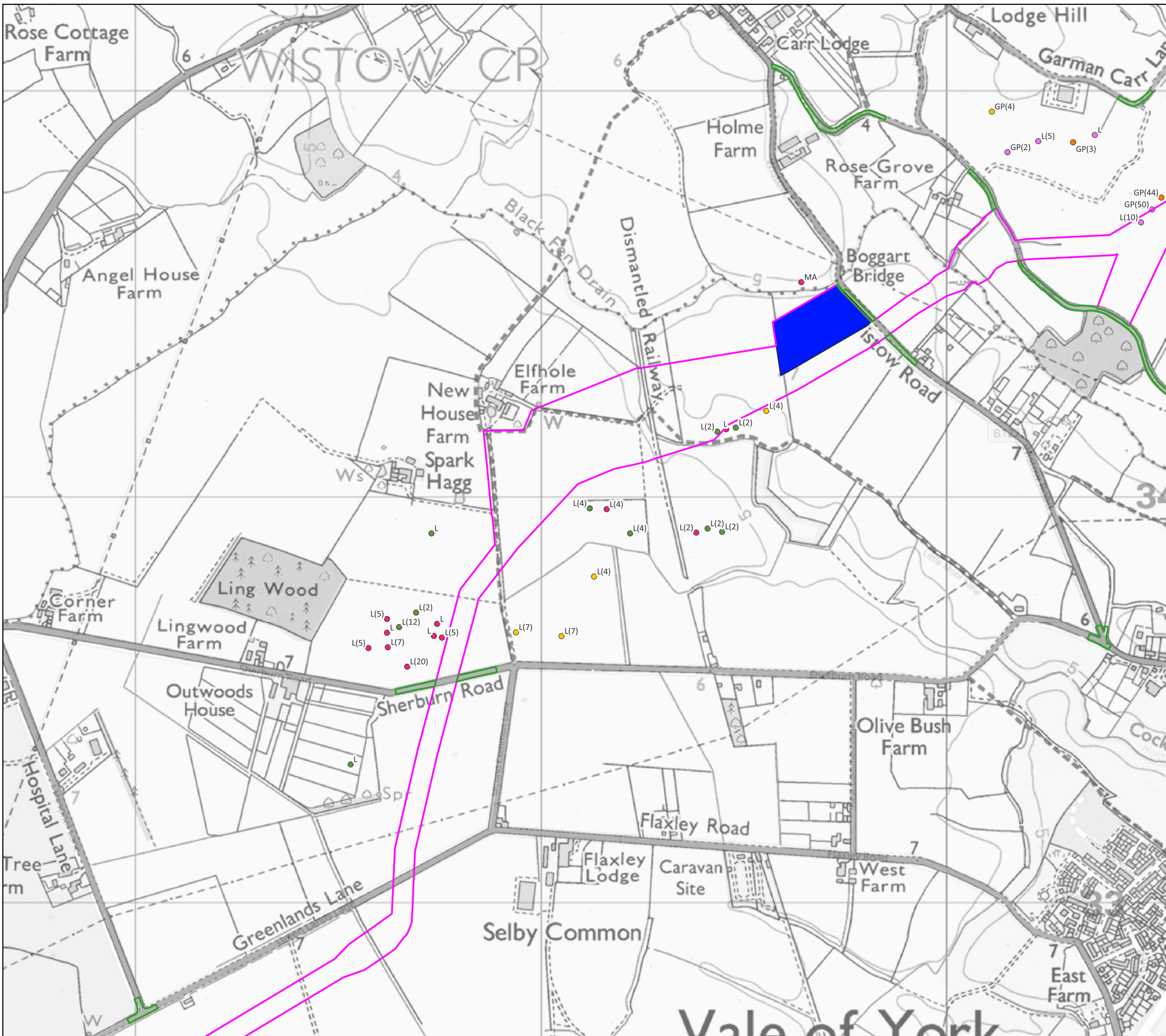
Figure 18: Non-Breeding Bird Results - Birds on the Ground Cable Route - Map 6
