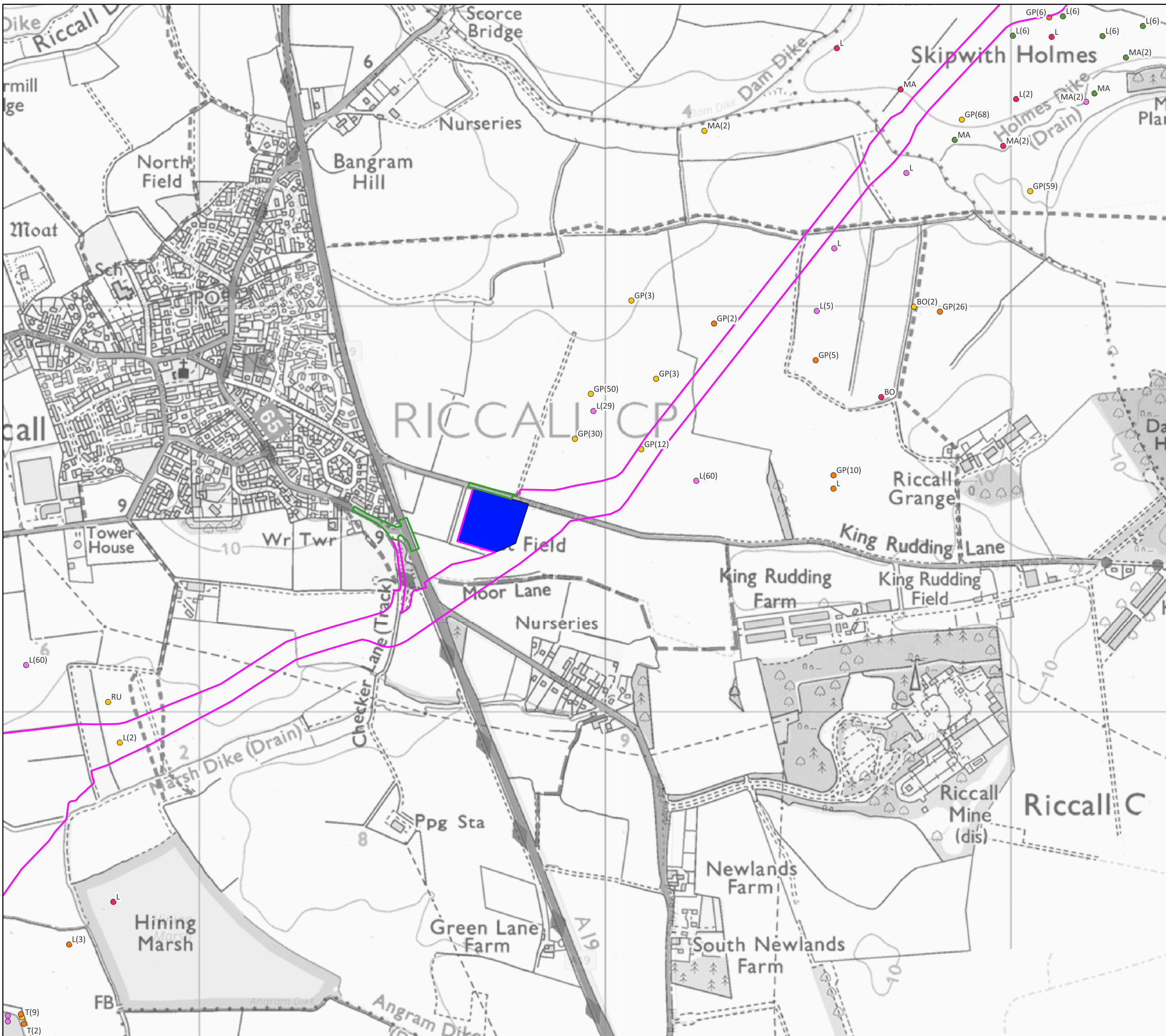
Figure 15: Non-Breeding Bird Results - Birds on the Ground Cable Route - Map 3
