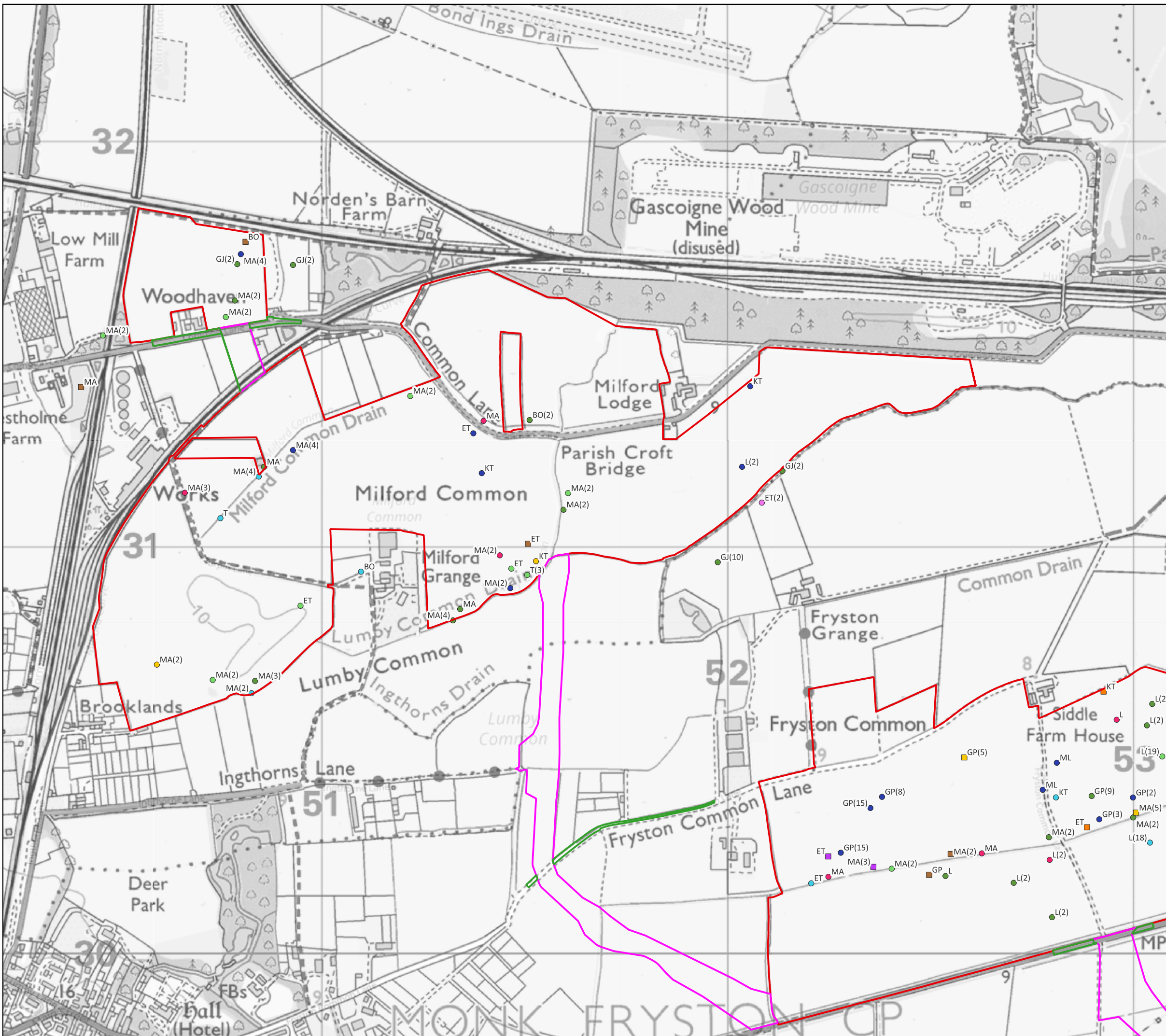
Figure 11: Non-Breeding Bird Results - Birds on the Ground Solar Development Site 6 & 7
