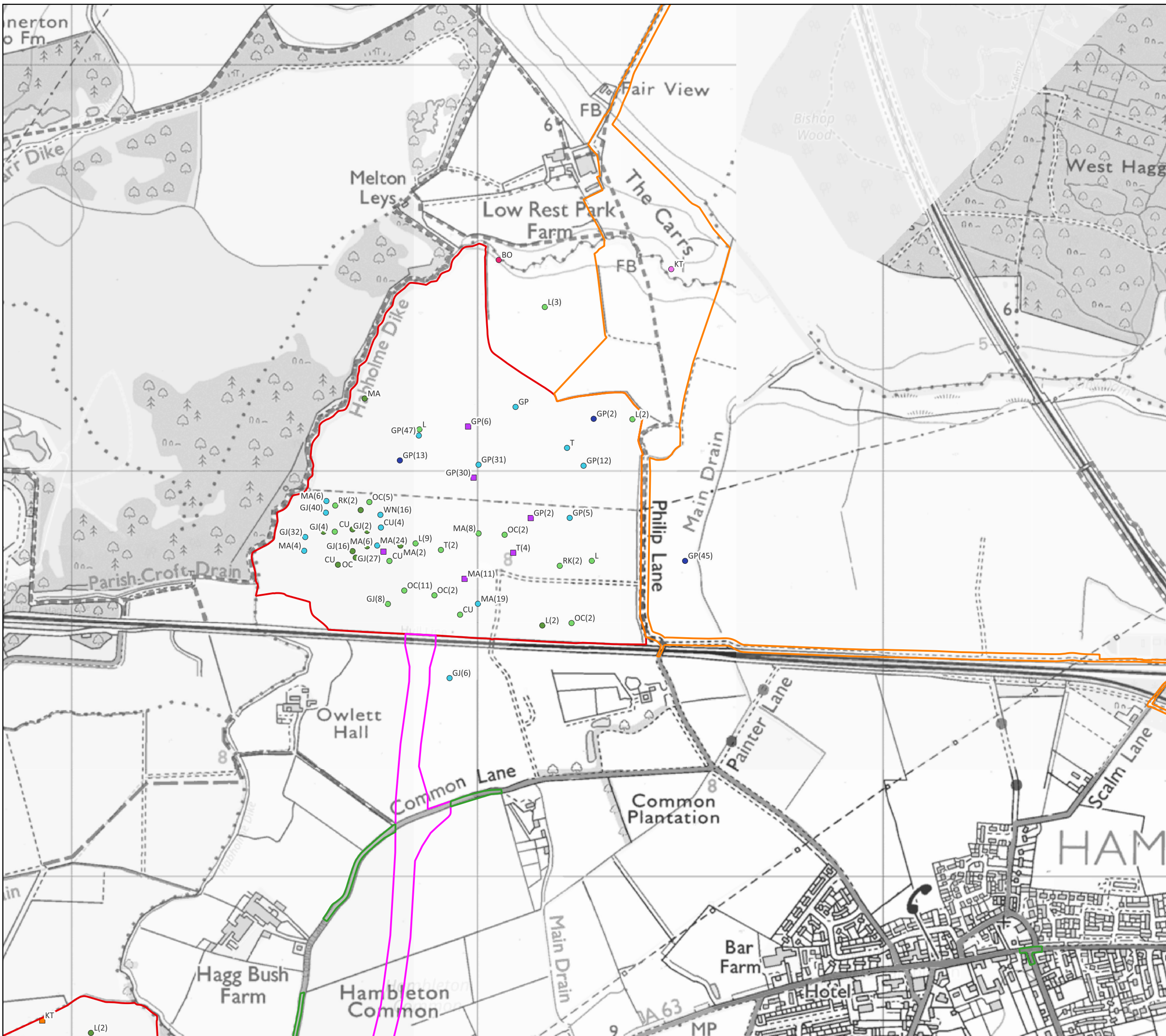
Figure 12: Non-Breeding Bird Results - Birds on the Ground Solar Development Site 8
